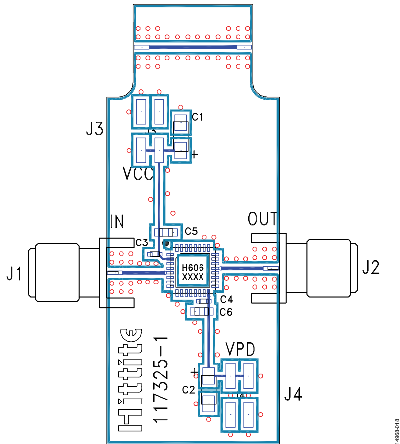
Figure 17. Evaluation PCB
