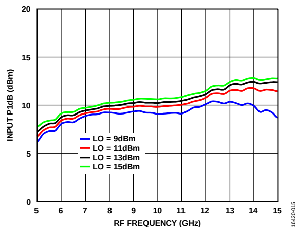
Figure 13. Input P1dB vs. RF Frequency at Various LO Power Levels, T_A = 25^\circ\text{C}
