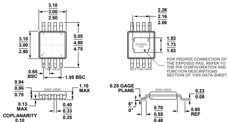
Figure 53. 8-Lead Mini Small Outline Package with Exposed Pad [MINI_SO_EP] (RH-8-1)
