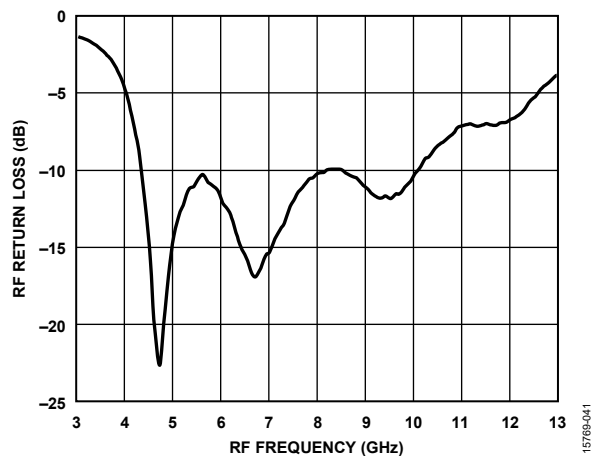
Figure 41. RF Return Loss vs. RF Frequency
