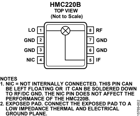
Figure 2. Pin Configuration
