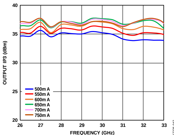
Figure 42. Output IP3 vs. Frequency for Various Quiescent Currents ( I_{DDQ} ), V_{DDx} = 5\text{ V}
