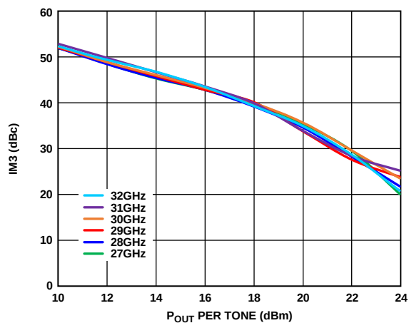
Figure 43. IM3 vs. P_{OUT} per Tone, V_{DDx} = 5\text{ V} , I_{DDQ} = 650\text{ mA}
