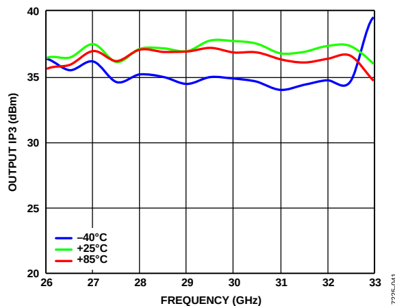
Figure 41. Output IP3 vs. Frequency for Various Temperatures, P_{OUT} per Tone = 20 dBm, V_{DDx} = 5\text{ V} , I_{DDQ} = 650\text{ mA}
