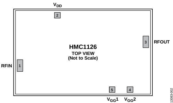
Figure 2. Pad Configuration
