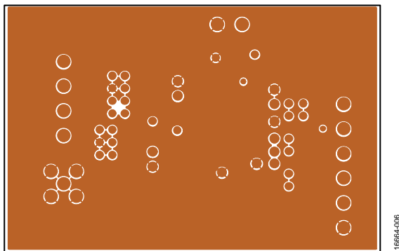
Figure 6. EVAL-ADM3067EEBZ, Layer 2
