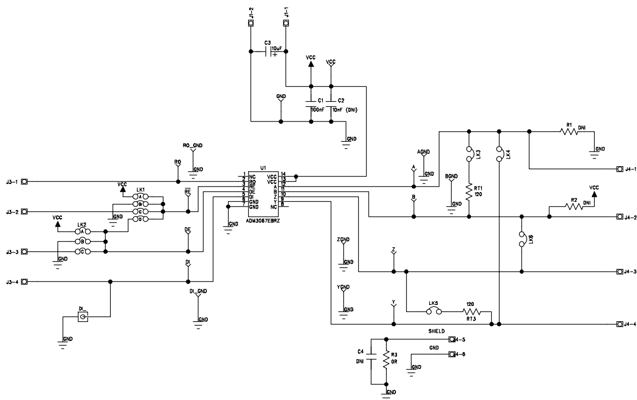
Figure 4. EVAL-ADM3067EEBZ Schematic
