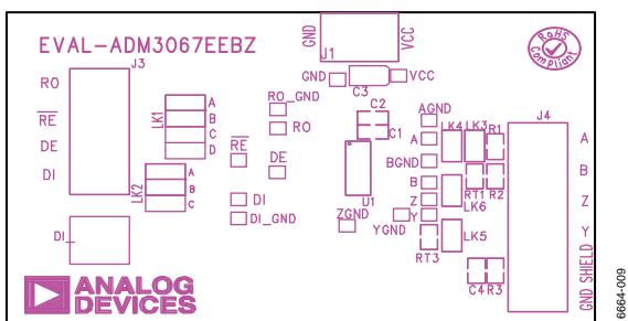
Figure 9. EVAL-ADM3067EEBZ, Silkscreen
