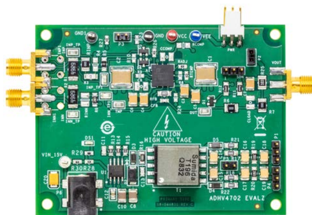
Figure 1. Evaluation Board, Top
