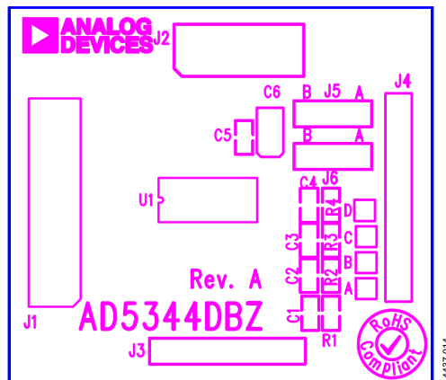
Figure 14. EVAL-AD5344DBZ Daughter Board Component Placement
