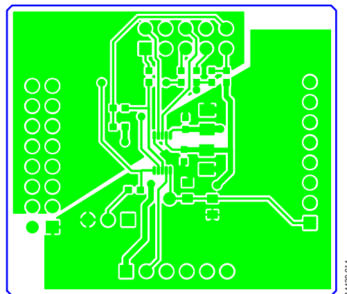
Figure 16. EVAL-AD5311RDBZ Daughter Board Top Side Routing
