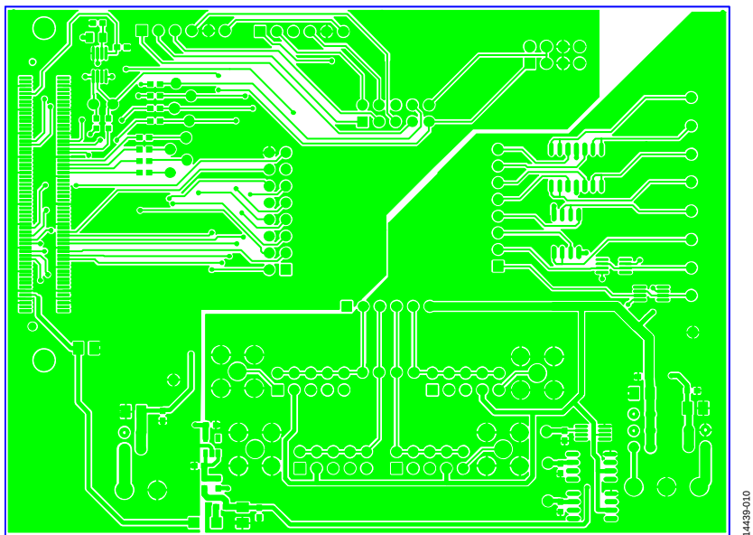
Figure 12. EVAL-MBnanoDAC-SDZ Motherboard Top Side Routing
