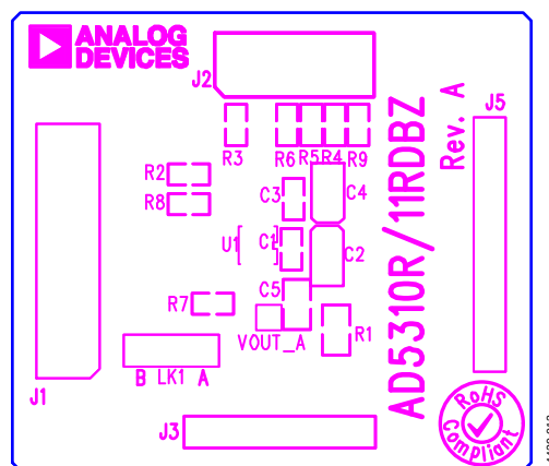
Figure 15. EVAL-AD5311RDBZ Daughter Board Component Placement
