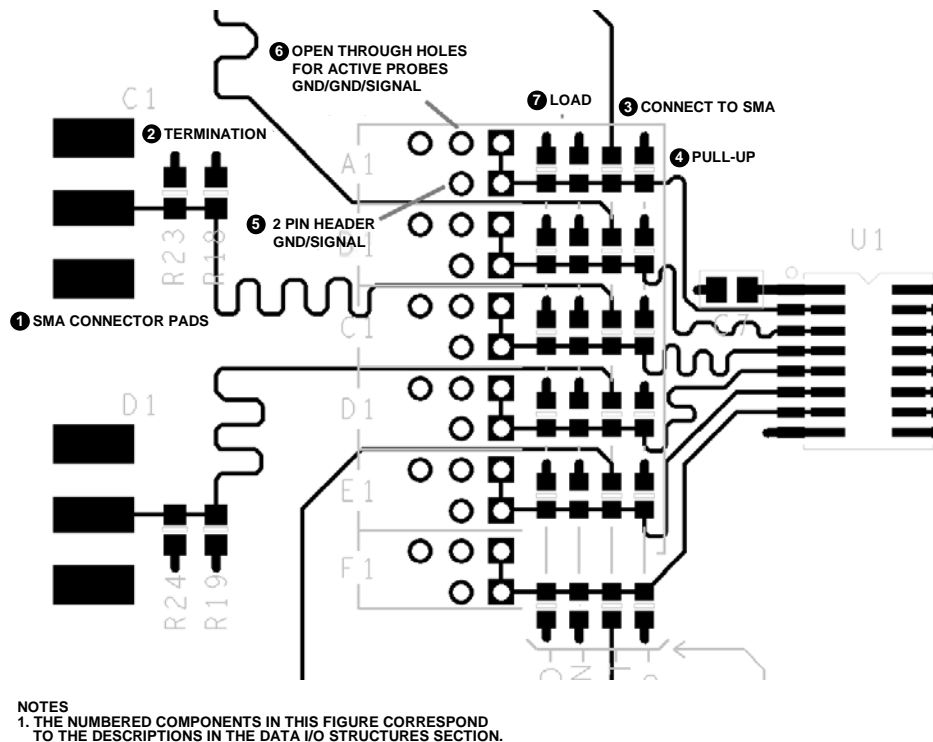
Figure 3. Configuration and Monitoring Structures
