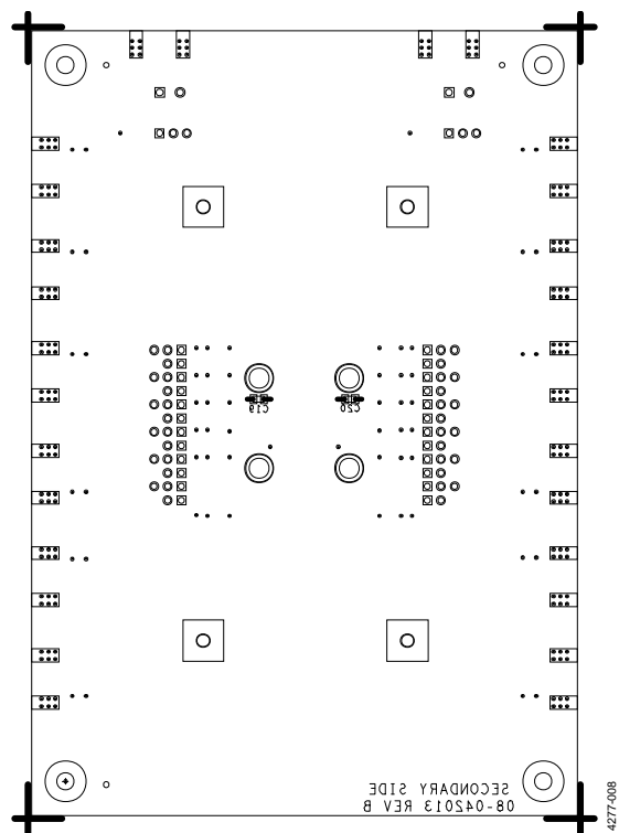
Figure 8. Bottom Layer Assembly and Routing (Layer 4)
