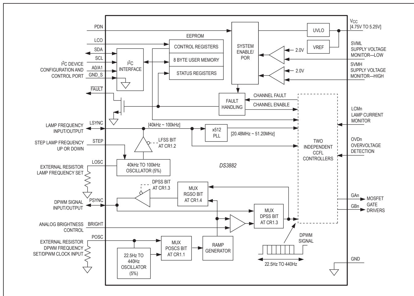
Figure 1. Functional Diagram
