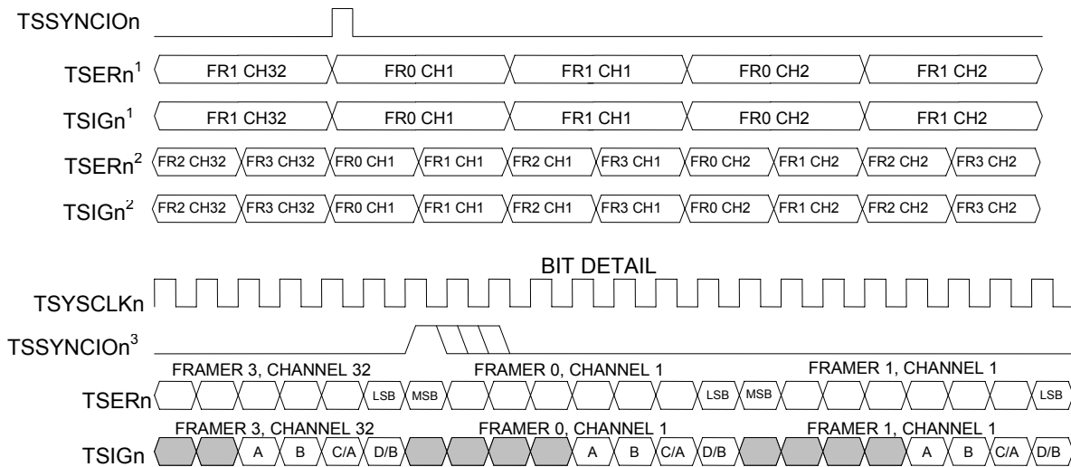
Figure 11-28. E1 Transmit-Side Interleave Bus Operation—BYTE Mode
