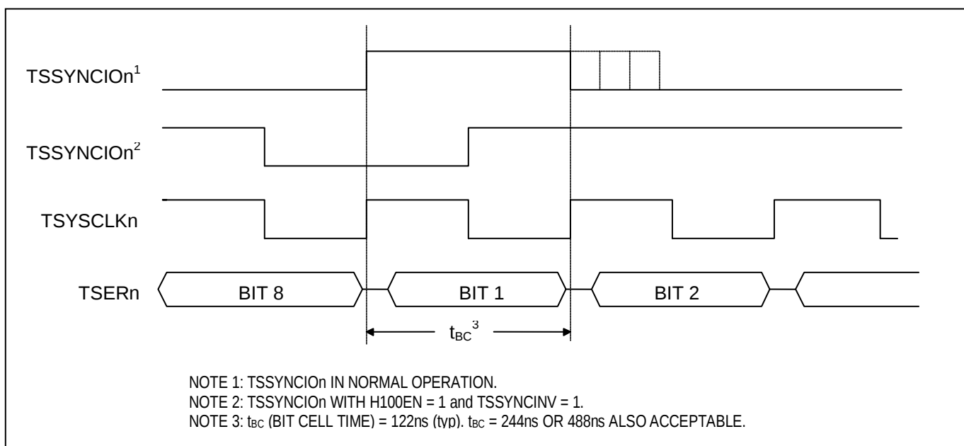
Figure 9-15. TSSYNCIOn (Input Mode) Input in H.100 (CT Bus) Mode
