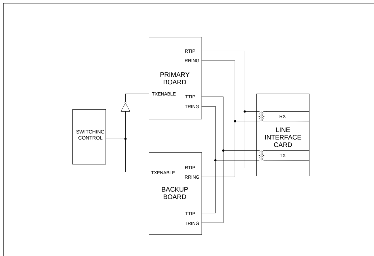
Figure 9-26. HPS Block Diagram
