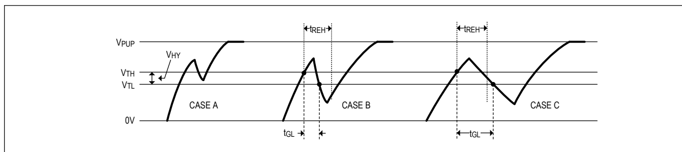
Figure 9. Noise Suppression Scheme
