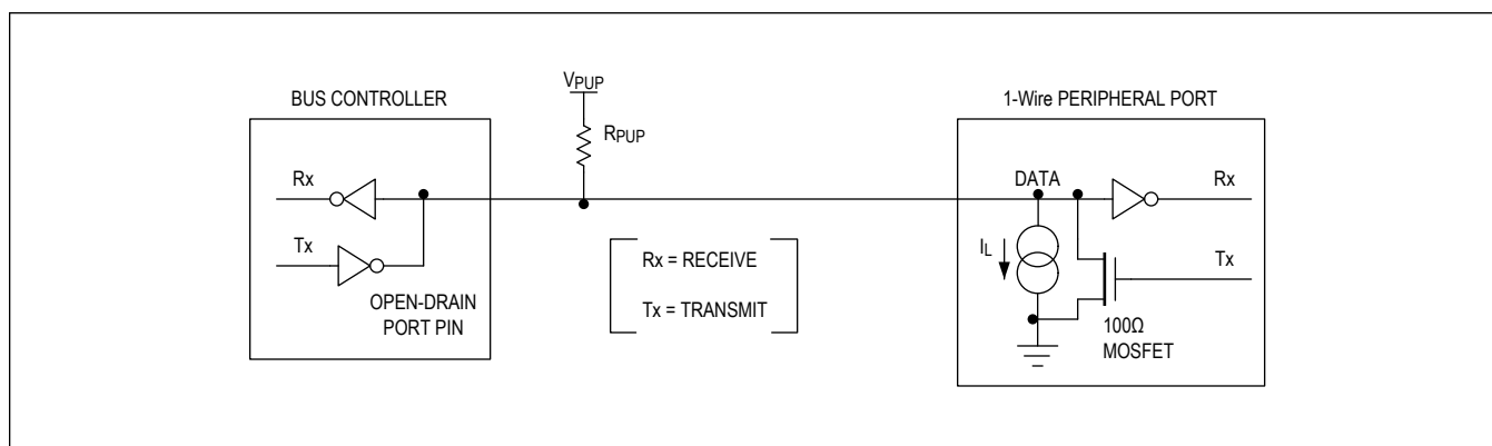
Figure 5. Hardware Configuration
