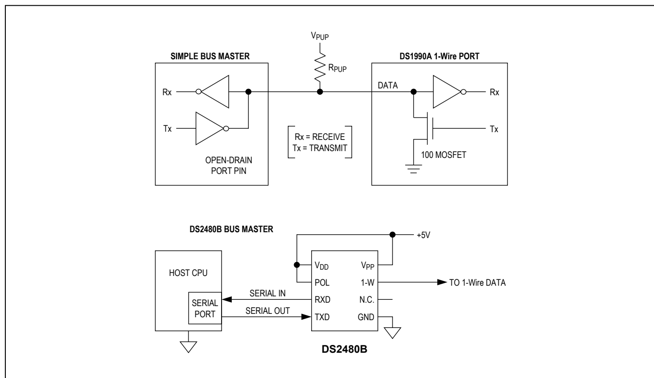
Figure 4. Hardware Configuration
