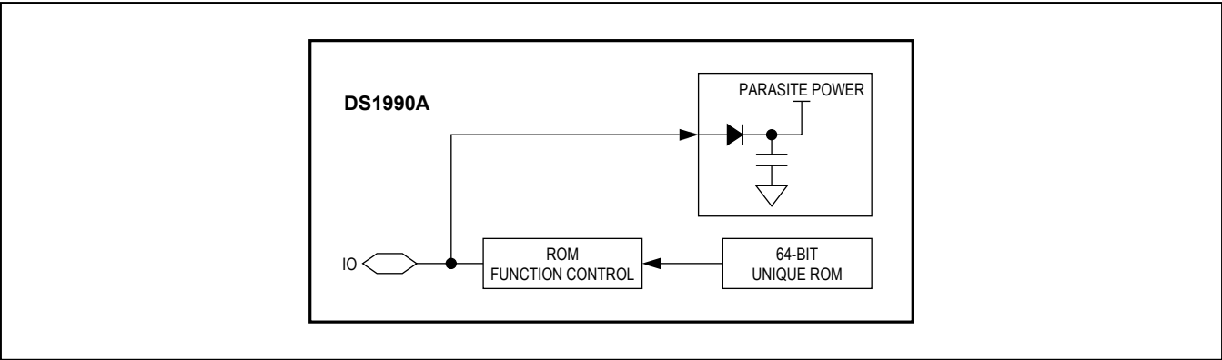
Figure 1. Block Diagram
