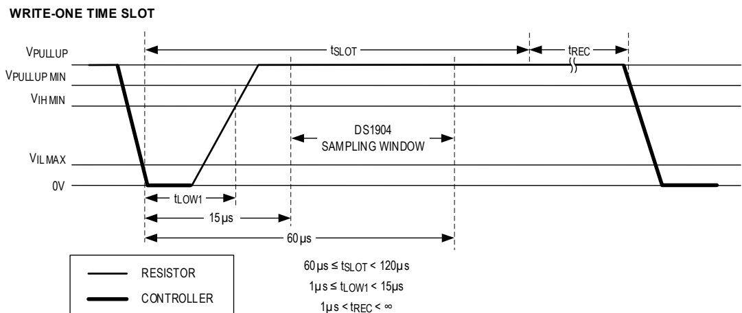
Read/Write Timing Diagram Figure 9
