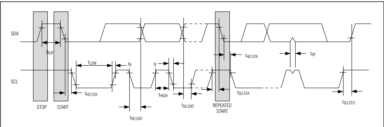
Figure 6. Timing Diagram
