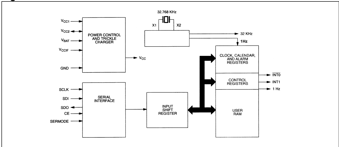
Figure 1. BLOCK DIAGRAM
