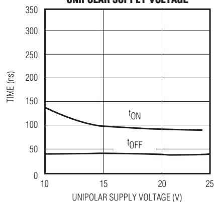
SWITCHING TIMES vs. UNIPOLAR SUPPLY VOLTAGE
