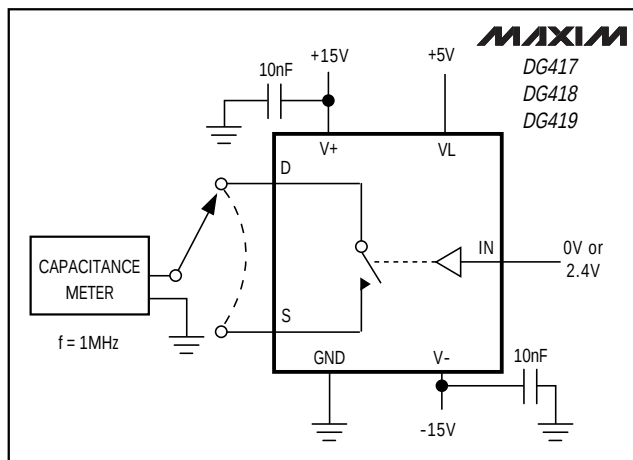
Figure 9. Drain-Source On-Capacitance
