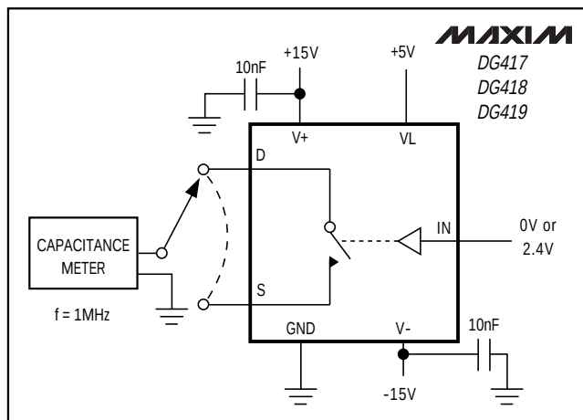
Figure 8. Drain-Source Off-Capacitance
