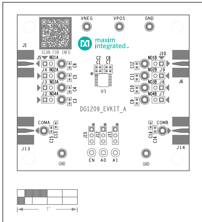
DG1209 EV Kit—Silkscreen Top
