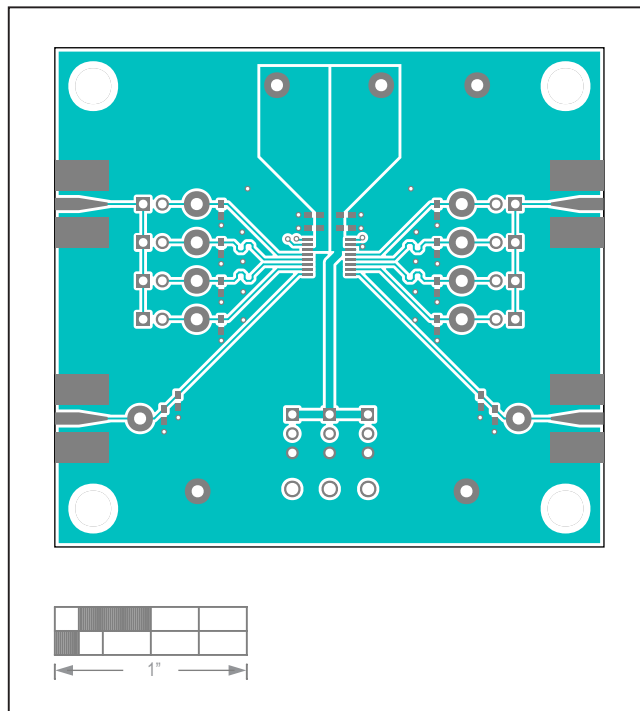
DG1209 EV Kit—Top Layer
