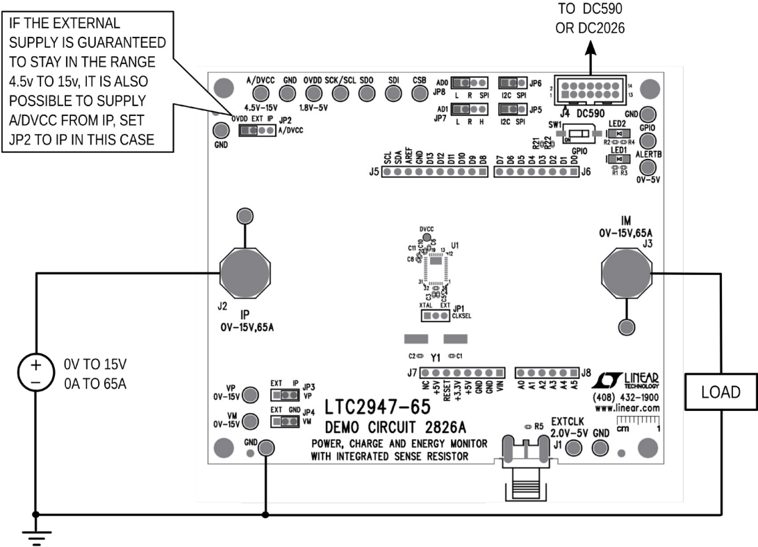
Figure 5. DC2826A Powered by DC590/DC2026 and Configured for High Side Sensing
