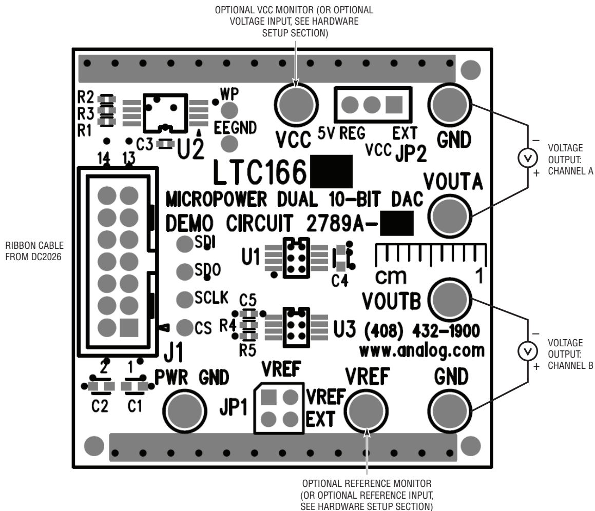
Figure 1. Connection Diagram
