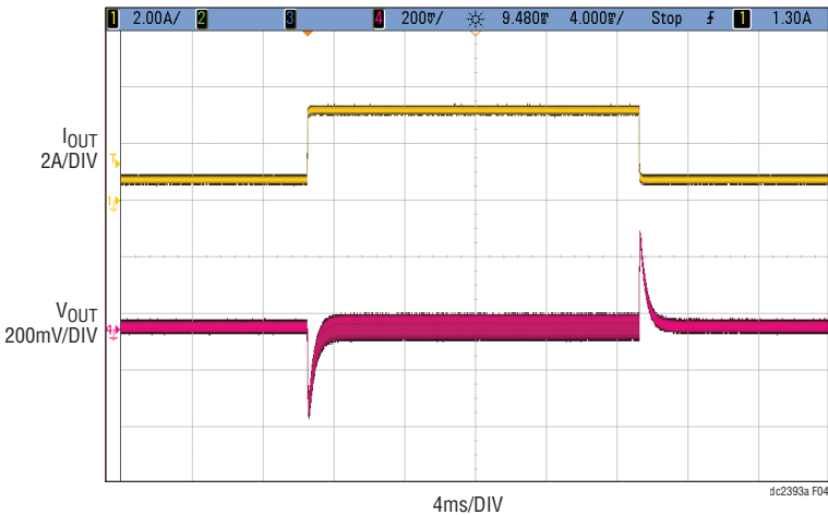
Figure 4. Load Transient Responses (V IN = 48V, Load Transient Between 1A and 3.5A)
