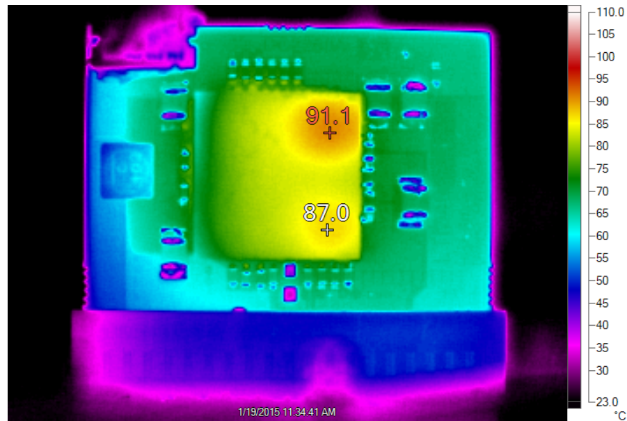
Figure 11. Thermal Performance at V_{IN} = 12V , V_{OUT0} = 1V/11A , V_{OUT1} = 1.8V/11A , f_{SW} = 500kHz , T_A = 23^\circ C , 200LFM Airflow
