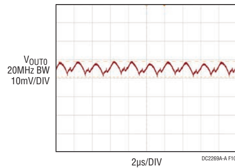
Figure 10. Output Voltage Ripple at V_{IN} = 12V , V_{OUT0} = 1.8V , I_{OUT0} = 13A
