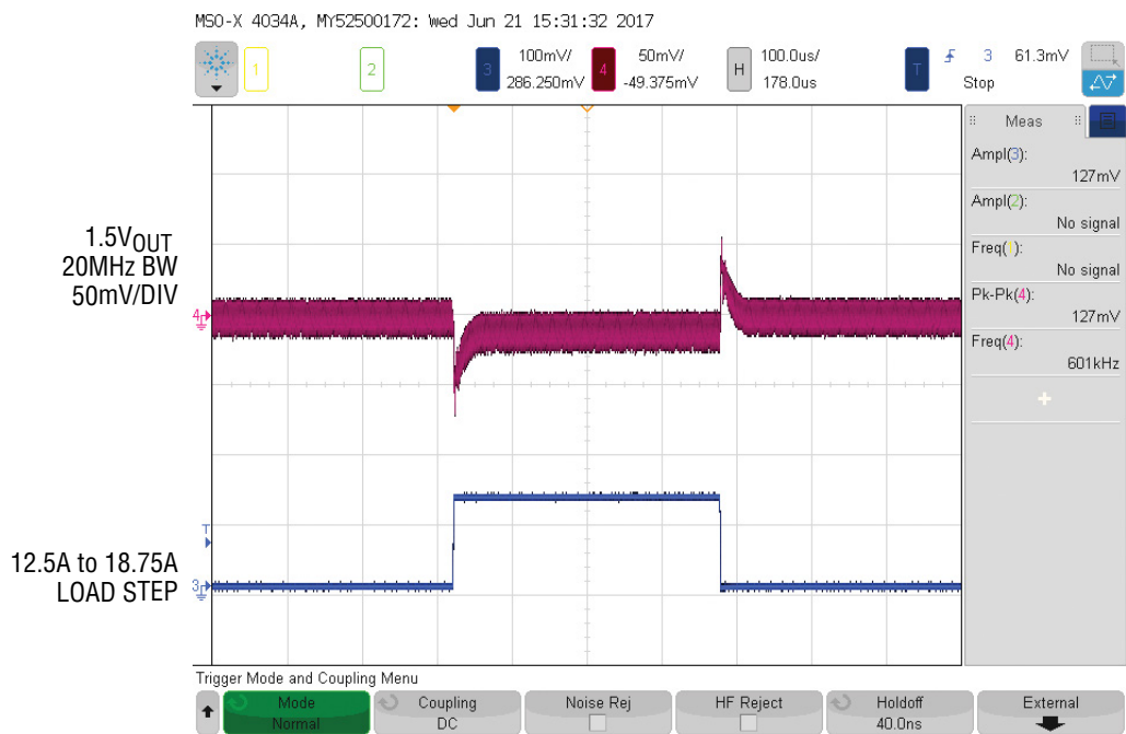
Figure 6. Measured Channel 12.5A to 18.75A Load Transient ( V_{IN} = 12V , V_{OUT2} = 1.5V )
