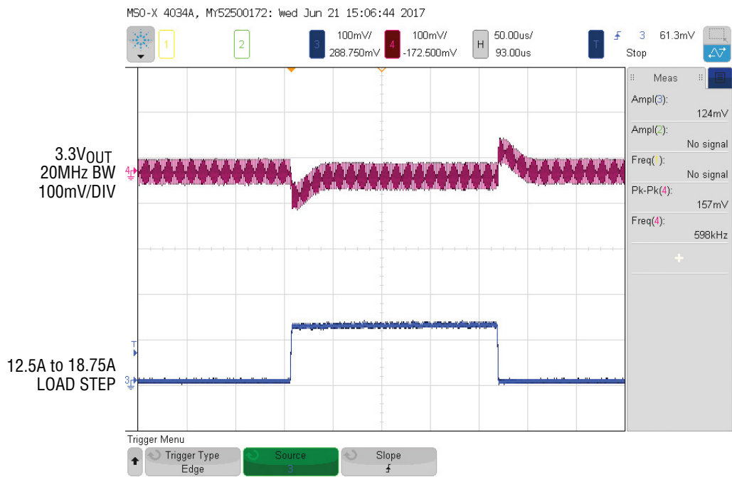
Figure 5. Measured Channel 1 12.5A to 18.75A Load Transient ( V_{IN} = 12V , V_{OUT1} = 3.3V )
