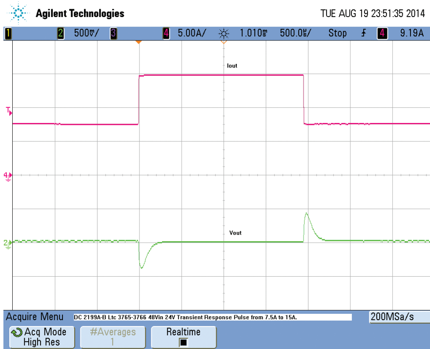
Figure 4. Transient Response Waveform at 48V IN and 7.5A to 15A to 7.5A OUT (5A, 500mV, 500μs/DIV)
