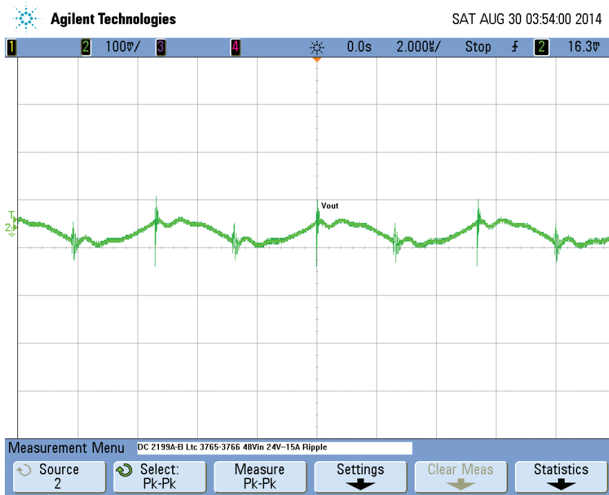
Figure 3. Output Ripple at 48V IN and 15A OUT (100mV, 2μs/DIV, 20MHz)
