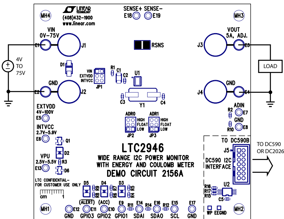
Figure 3a. DC2156A Is Powered from V_{IN}
