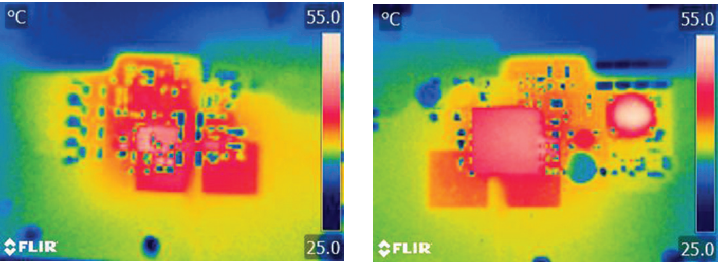
Figure 1. Thermal Pictures – V_{PORT} = 42.5V, 5V/4.7A
