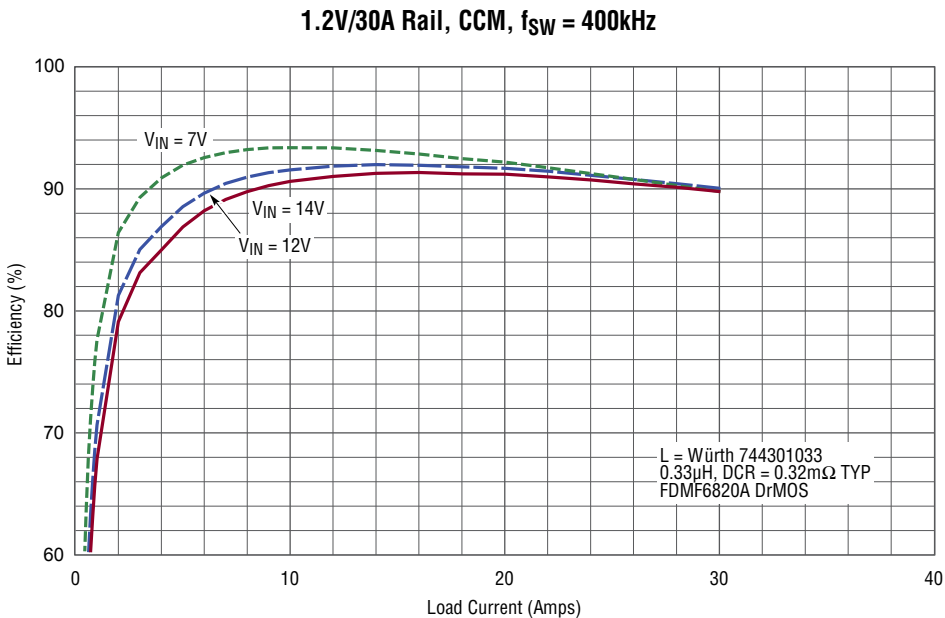
Figure 3. Efficiency Curves for the 1.2V Rail at V_{IN} = 12V , 14V and 7V in CCM.
