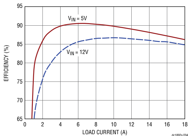
Figure 4. Measured Efficiency on Channel 2. V_{OUT2} = 1V , f_{sw} = 500kHz , Channel 1 Disabled, CCM, 0A to 18A
