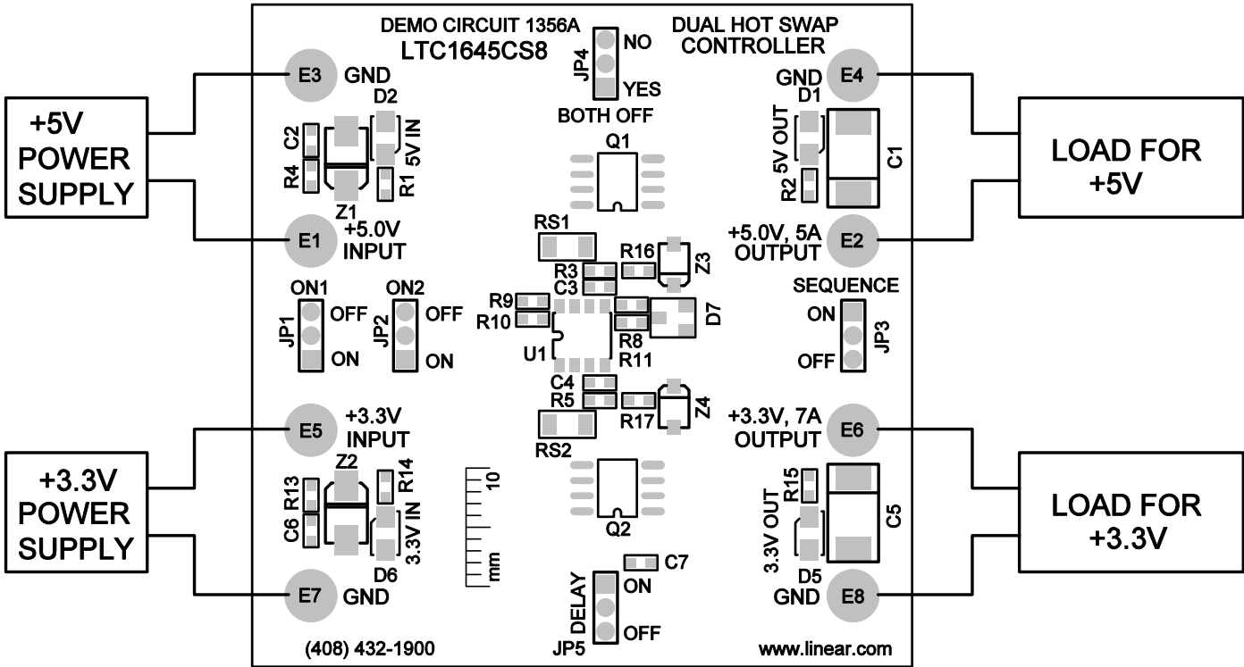
Figure 1. DC1356A Measurement Equipment Setup
