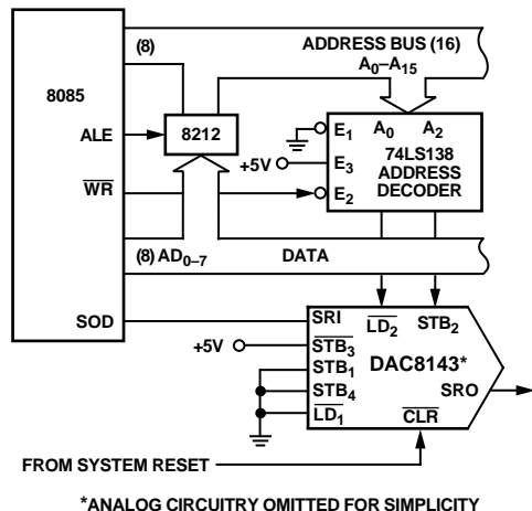
Figure 22. DAC8143—8085 Interface
