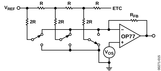
Figure 15. Simplified Circuit
