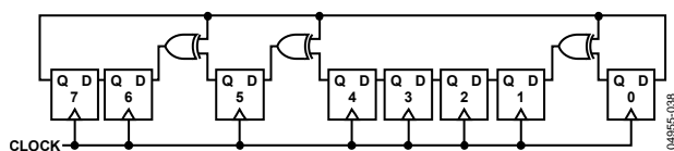
Figure 81. 8-Bit LFSR
