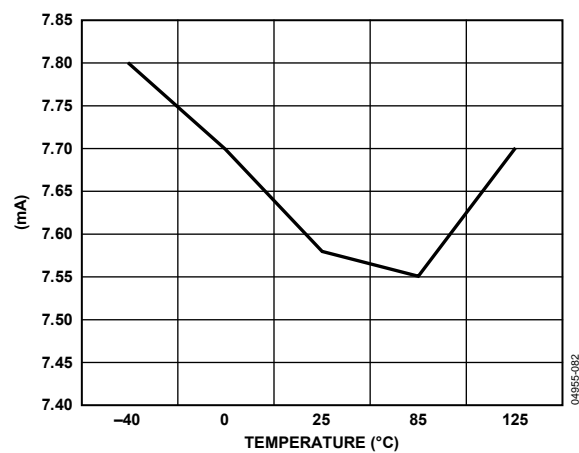
Figure 41. Current Consumption vs. Temperature @ CD = 7
