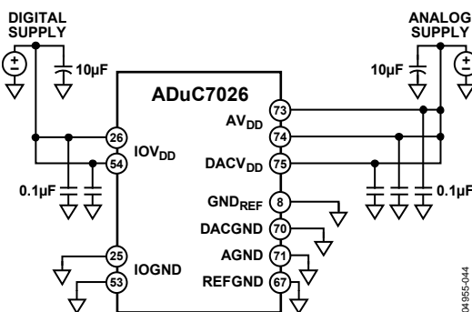
Figure 87. External Dual Supply Connections
