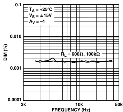
TPC 6. Dynamic Intermodulation Distortion vs. Frequency
