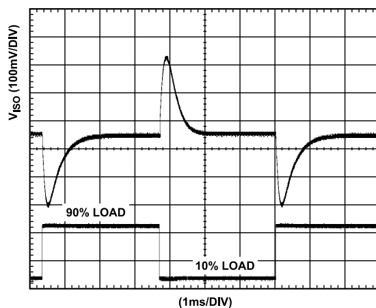
Figure 10. Typical V_{ISO} Transient Load Response, 5 V Output, 10% to 90% Load Step
