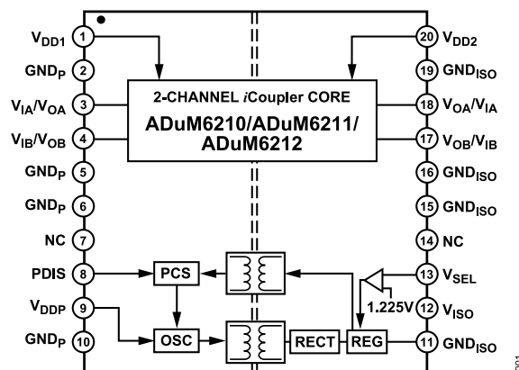
Figure 1. ADuM6210/ADuM6211/ADuM6212
