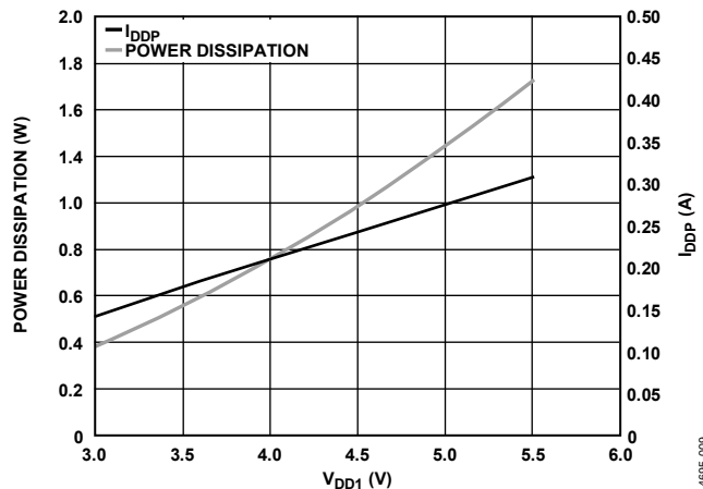
Figure 9. Short-Circuit Input Current ( I_{DDP} ) and Power Dissipation vs. V_{DD1} Supply Voltage
