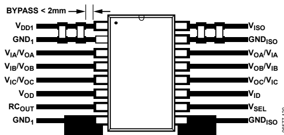
Figure 25. Recommended PCB Layout
