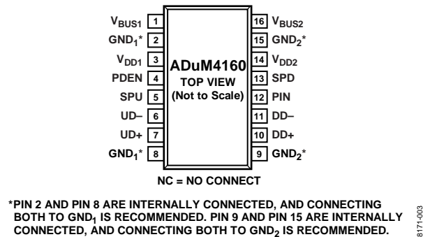
Figure 3. Pin Configuration
