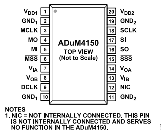
Figure 3. Pin Configuration
