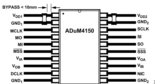
Figure 14. Recommended PCB Layout
