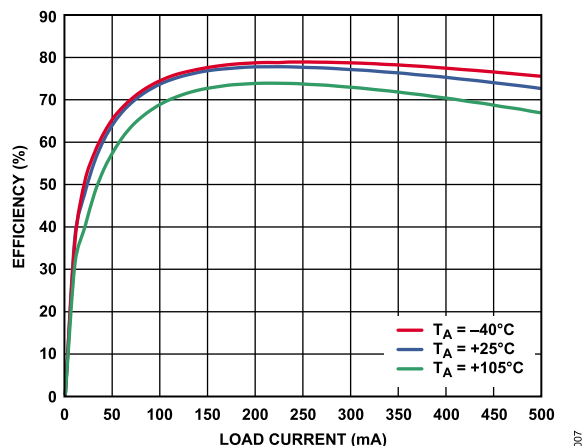
Figure 7. Typical Efficiency over Temperature with 1:2 Coilcraft Transformer (CR7983-CL), f_{SW} = 500\text{kHz} , 5 V Input to 5 V Output
