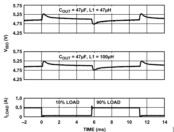
Figure 20. Typical V_{ISO} Load Transient Response at 10% to 90% of 500 mA Load with 0.1 \mu F Feedback Capacitor, f_{SW} = 500 kHz, 5 V Input to 5 V Output
