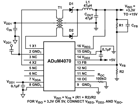
Figure 31. Single Power Supply
