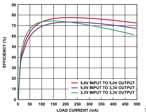
Figure 8. Single-Supply Efficiency with 1:2 Coilcraft Transformer (CR7983-CL), f_{SW} = 500\text{kHz}
