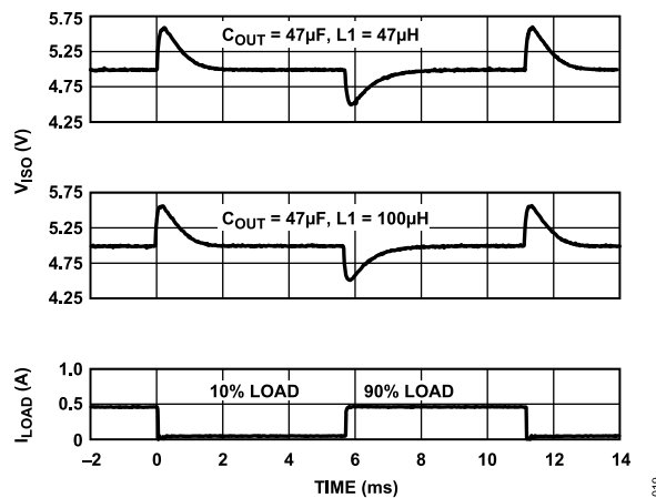
Figure 19. Typical V_{ISO} Load Transient Response at 10% to 90% of 500 mA Load, f_{SW} = 500 kHz, 5 V Input to 5 V Output
