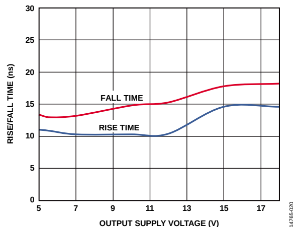
Figure 13. Rise/Fall Time vs. Output Supply Voltage
