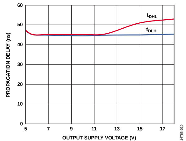
Figure 12. Propagation Delay vs. Output Supply Voltage, V_{DD1} = 5\text{ V}
