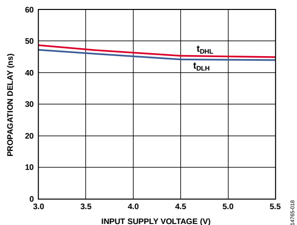
Figure 11. Propagation Delay vs. Input Supply Voltage, V_{DD2} = 10\text{ V}
