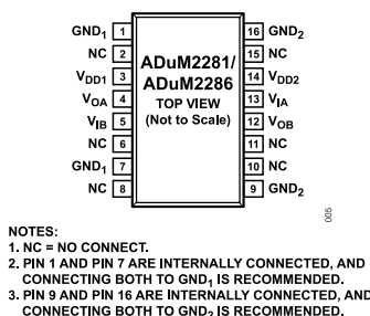
Figure 5. ADuM2281/ADuM2286 Pin Configuration
