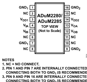
Figure 4. ADuM2280/ADuM2285 Pin Configuration
