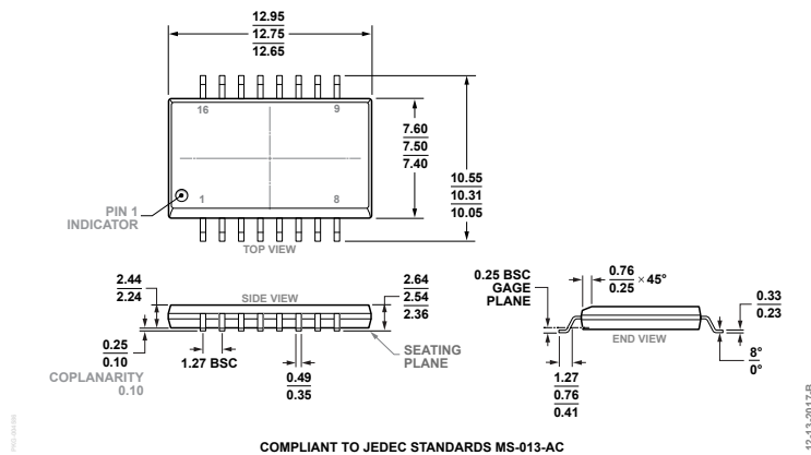
Figure 19. 16-Lead Standard Small Outline Package, with Increased Creepage [SOIC_IC] Wide Body (RI-16-2) Dimensions shown in millimeters
