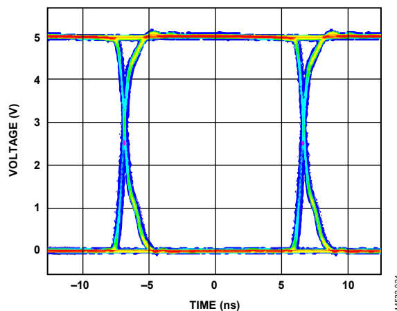
Figure 24. ADuM160N/ADuM161N/ADuM162N/ADuM163N Eye Diagram
