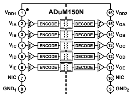
Figure 1. ADuM150N Functional Block Diagram
