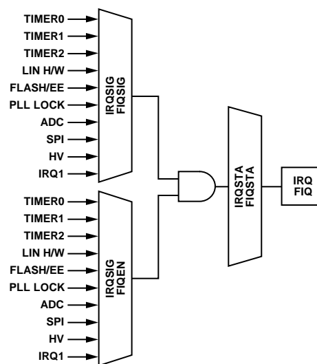
Figure 22. Interrupt Structure
