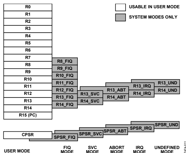
Figure 11. Register Organization
