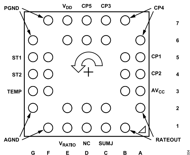
Figure 3. Pin Configuration
