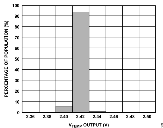
Figure 8. V_{TEMP} Output at 25°C ( V_{RATIO} = 5 V )
