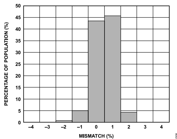
Figure 7. Self-Test Mismatch at 25°C ( V_{RATIO} = 5 V )
