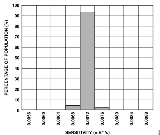
Figure 9. Sensitivity at 25°C
