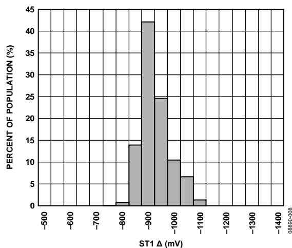
Figure 8. ST1 Output Change at 25°C ( V_{\text{RATIO}} = 5 \text{ V} )
